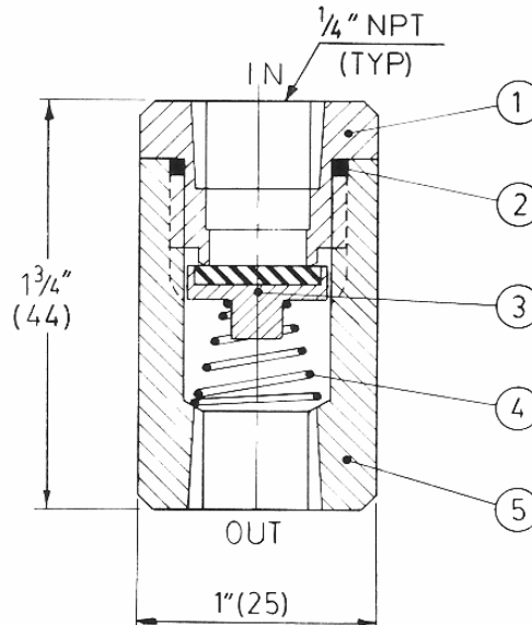
All dimensions in inches (mm)
