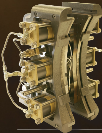
Hydraulic Applied Service Brakes
