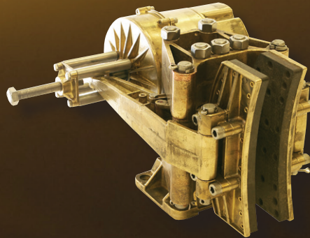
Spring Applied Emergency Brakes
