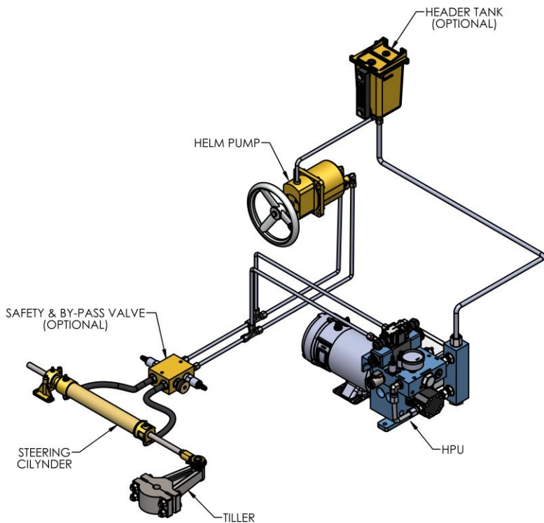
Figure 10: Typical System Arrangement, Closed Loop
