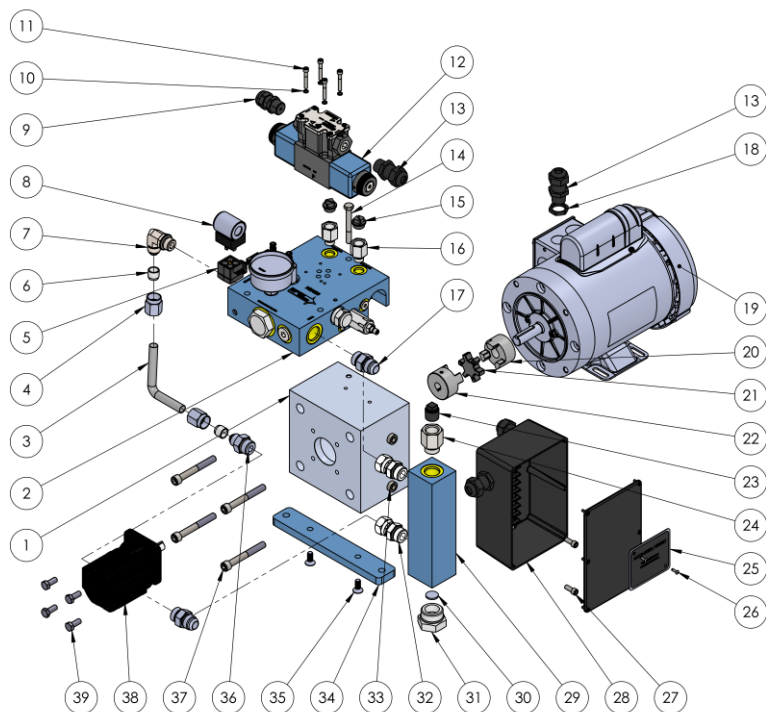
Figure 13: HPU300-AC Parts Diagram
