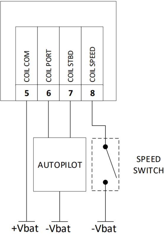
Figure 10: HPU300 Autopilot Wiring Diagram, Common Positive
