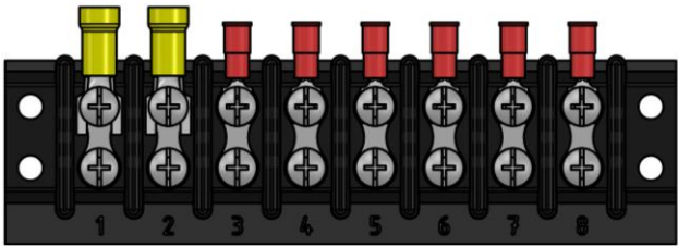
Figure 5: HPU300-DC Terminal Block Diagram
