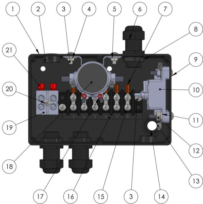
Figure 8: 503-023 ELECTRICAL BOX
