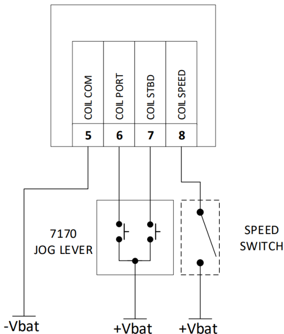
Figure 9: HPU300 Jog Control Diagram, Common Negative
