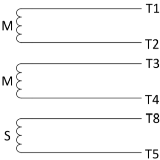
Figure 8: HPU300 AC Motor Wiring Diagram
