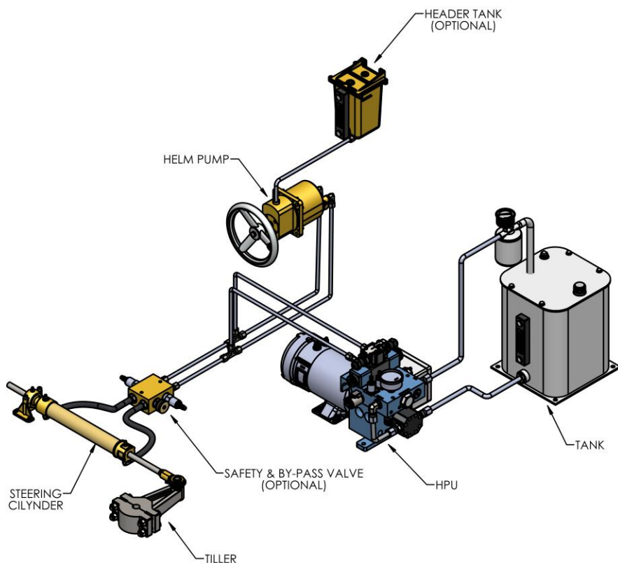
Figure 11: Typical System Arrangement, Open Loop
