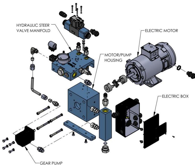
Figure 1: HPU300 Overview Diagram
