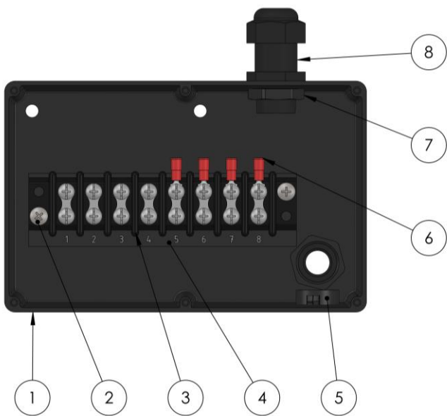
Figure 17: AC ELECTRICAL BOX
