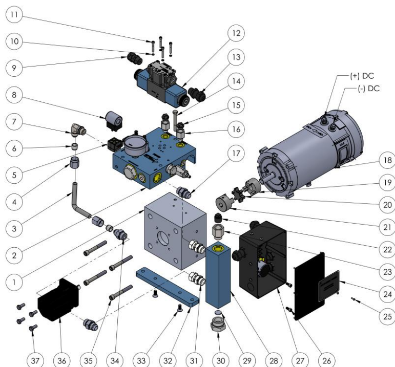
Figure 12: HPU300-DC Parts Diagram
