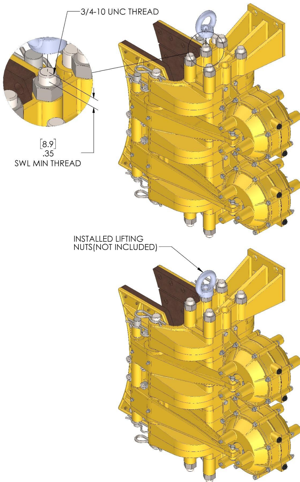
Figure 2: 5026-AW rigging
