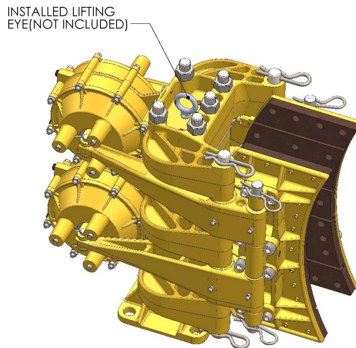
Figure 1: 5026-A rigging
