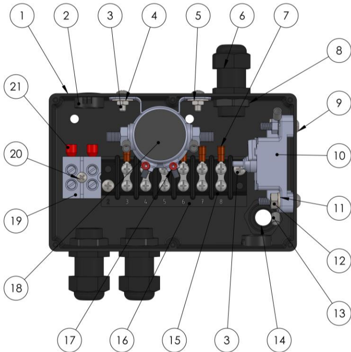
Figure 15: 503-025 ELECTRICAL BOX
