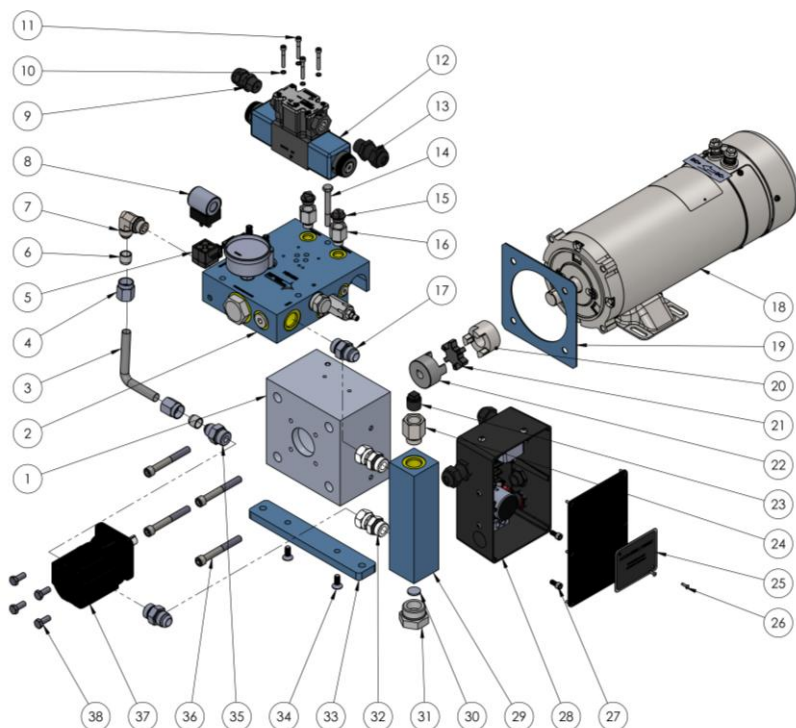
Figure 12: HPU400-24VDC Parts Diagram
