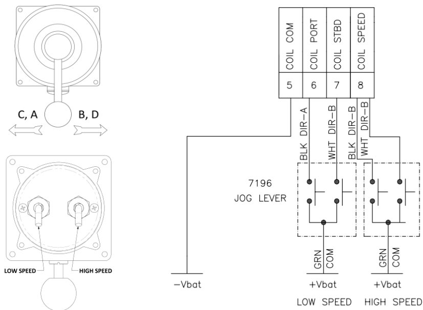
Figure 9: HPU400 7196 Jog Control Diagram, Common Negative
