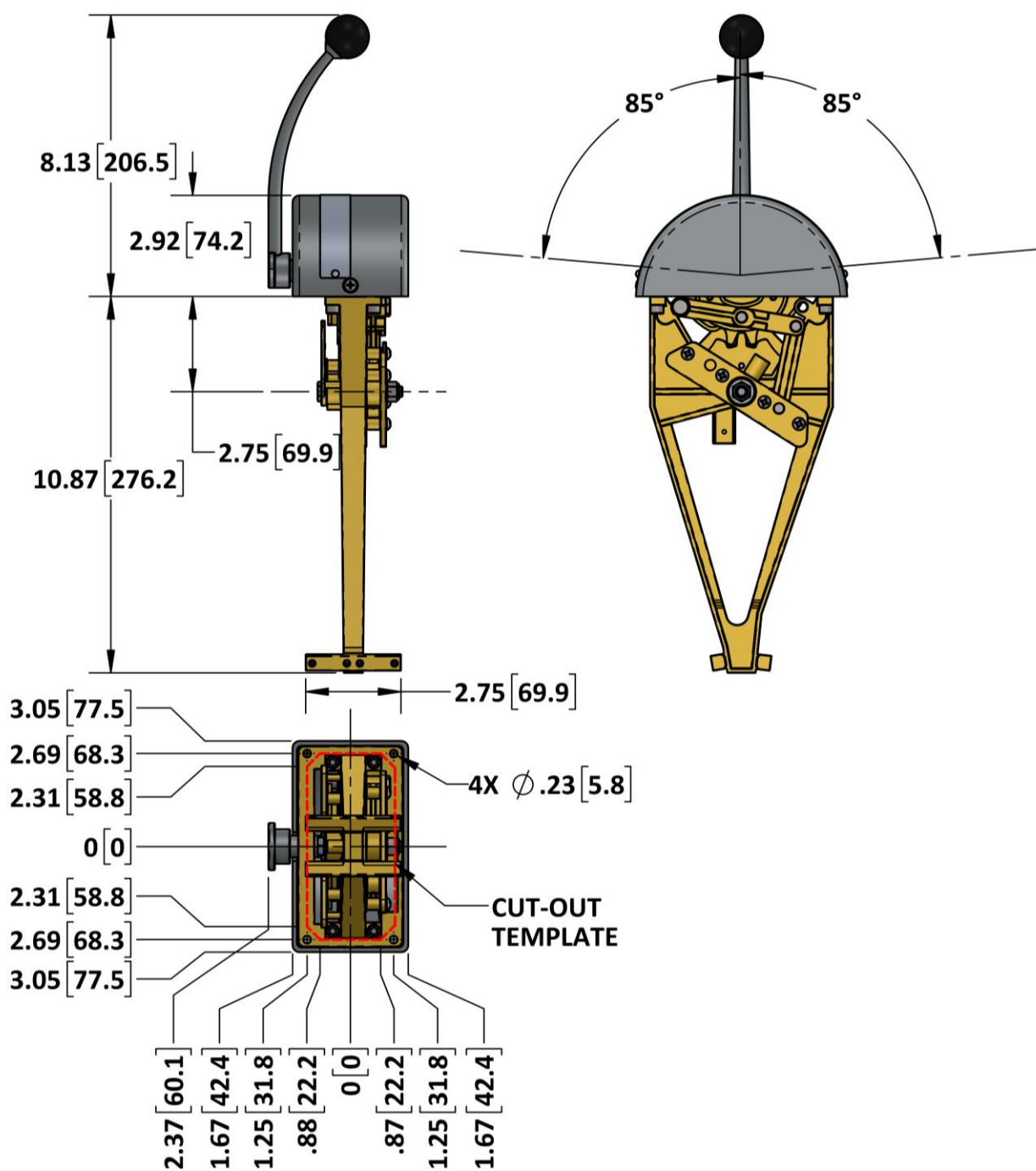
Figure 18: 2046 Installation Dimensions
