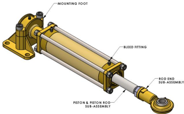
Figure 1: 7080 Cylinder Overview Diagram
