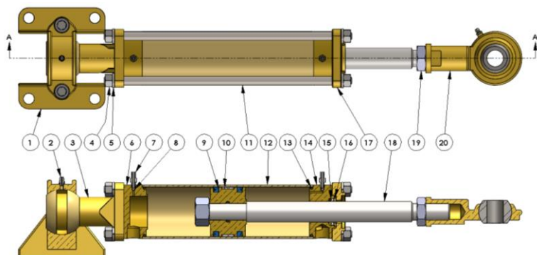
Figure 5: 7080 Unbalance Cylinder Parts Diagram
