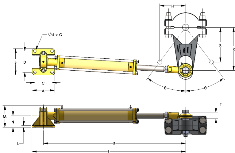
Figure 3: 7080 Unbalanced Cylinder Installation Diagram
