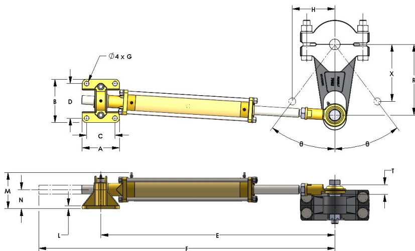
Figure 2: 7080 Balanced Cylinder Installation Diagram
