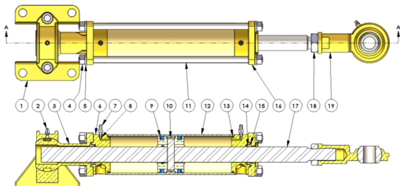
Figure 4: 7080 Balance Cylinder Parts Diagram
