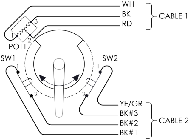
Figure 5: 7174-A wiring
