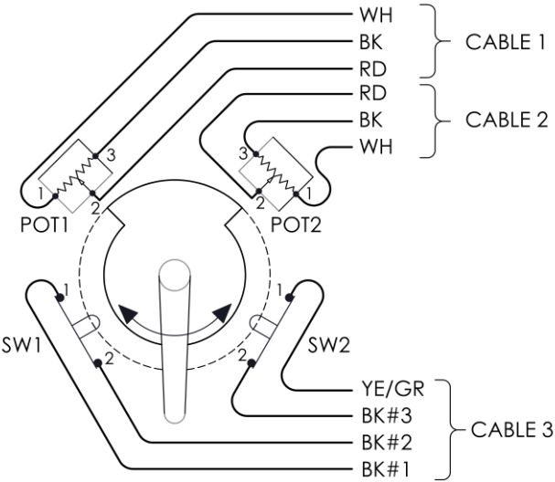
Figure 6: 7174-B wiring
