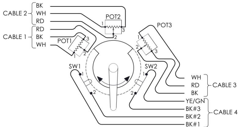
Figure 7: 7174-C wiring
