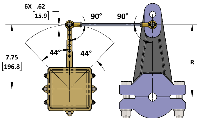
Figure 3: RFU Installation
