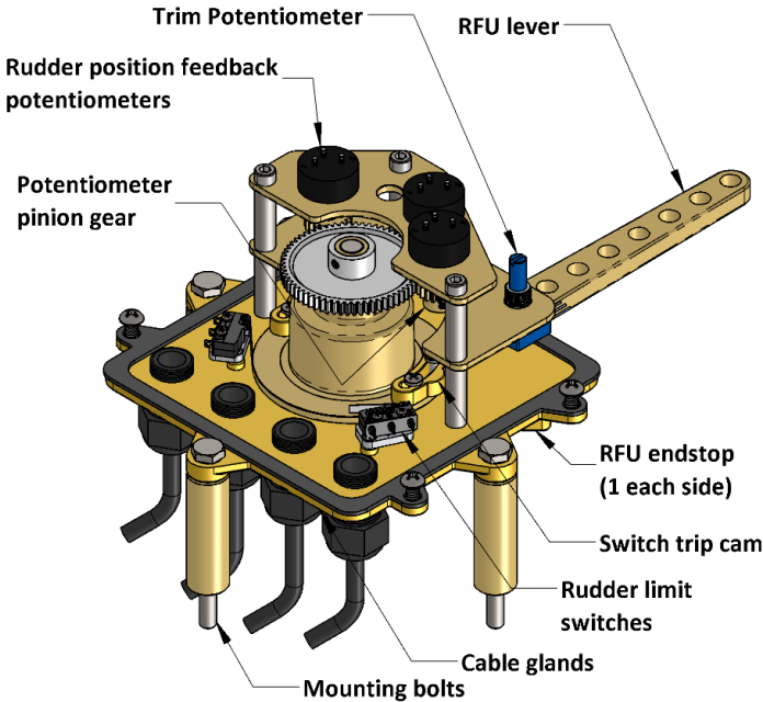
Figure 1: Product overview, 7174-CE shown.
