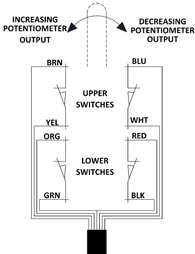
Figure 4: 7174-(J)G Limit Switch Wiring
