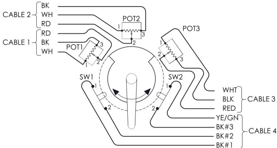
Figure 3: 7174-C wiring
