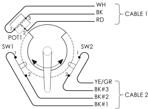
Figure 1: 7174-A wiring
