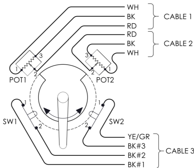
Figure 2: 7174-B wiring
